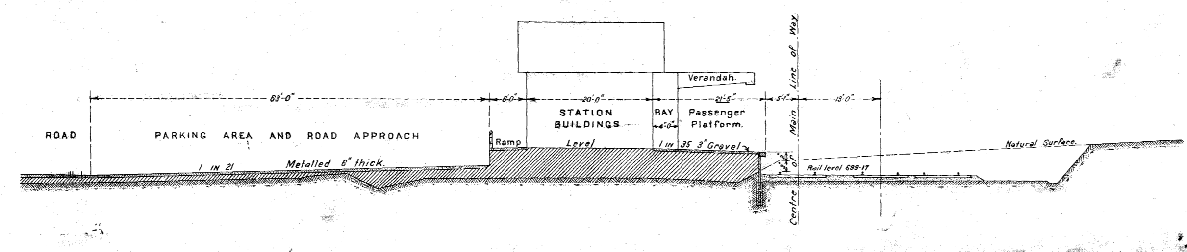
CROSS SECTION ON LINE A-A Scale 10 Feet = 1 Inch
