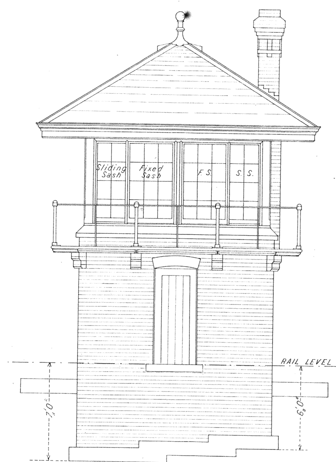
EAST ELEVATION
