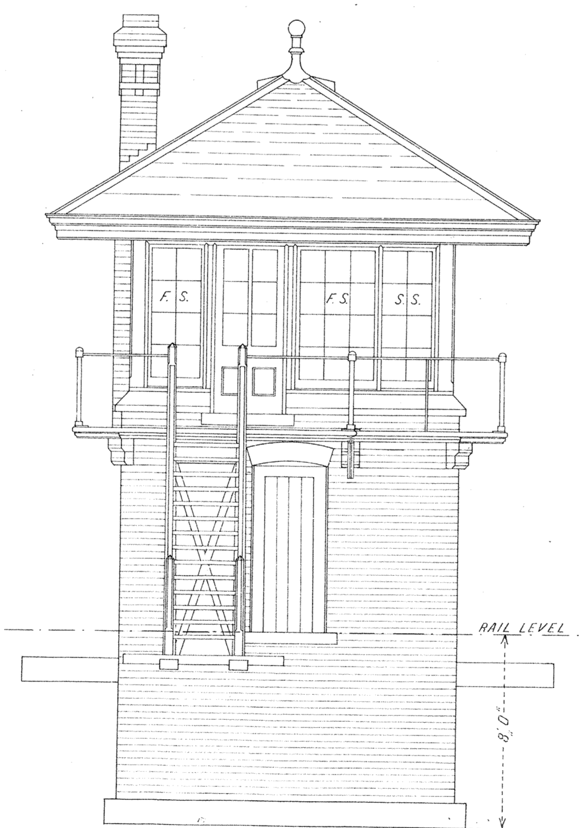
WEST ELEVATION
