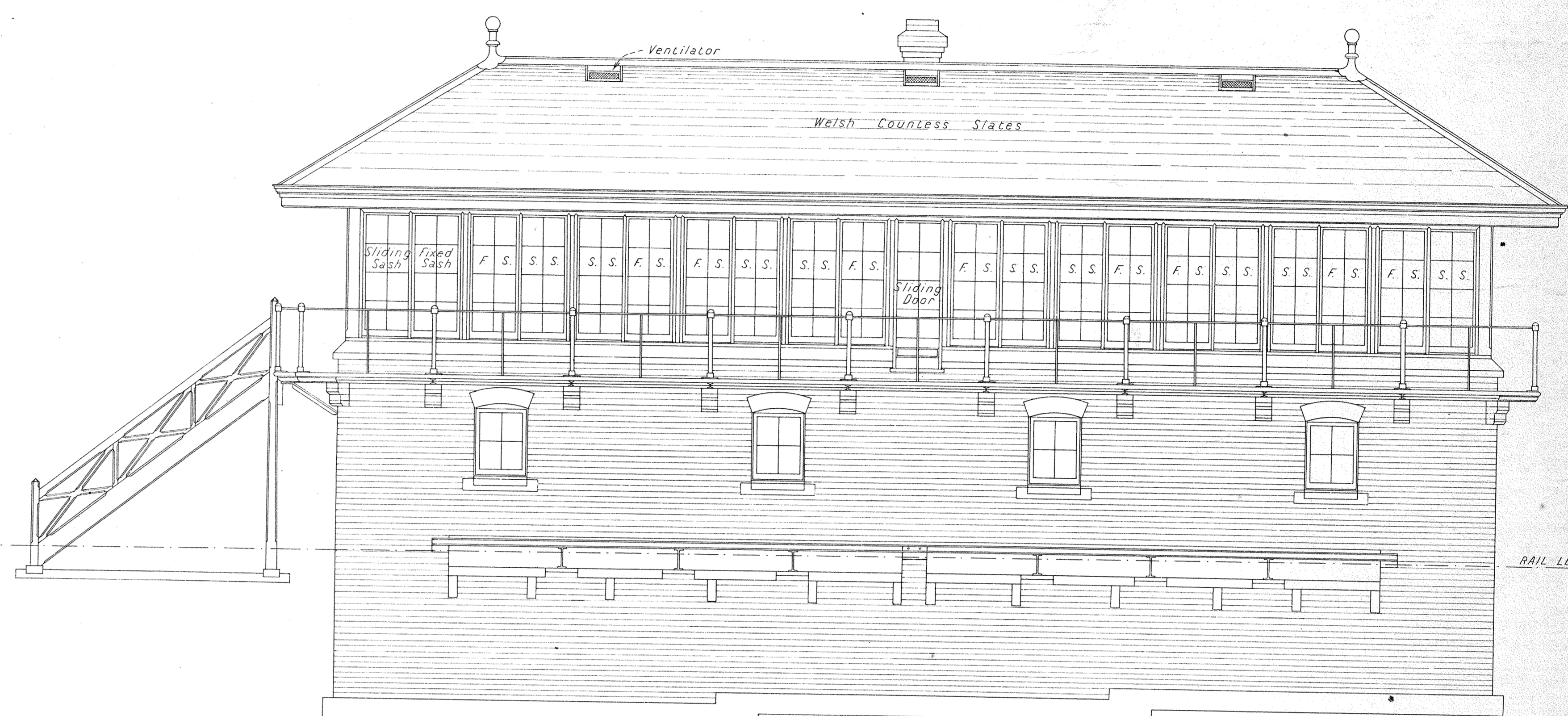
SOUTH ELEVATION
