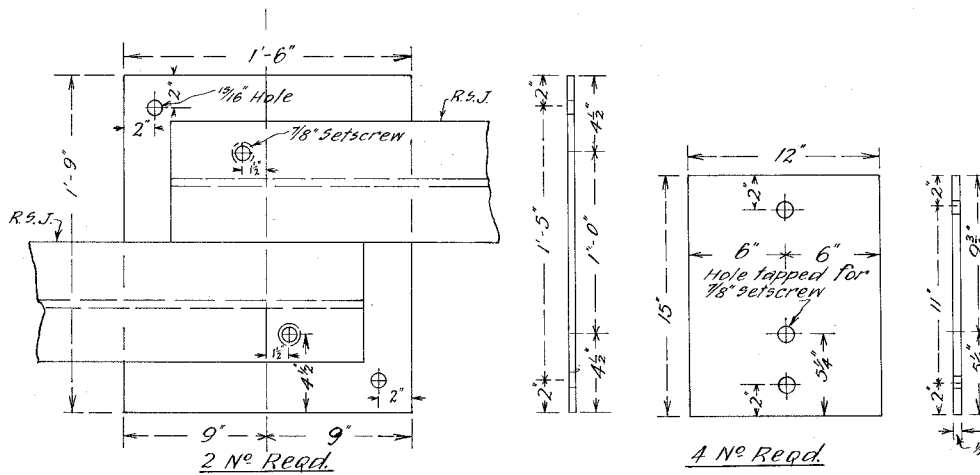
DETAILS OF BEDPLATES SCALE 1 1/2" = 1'-0"
