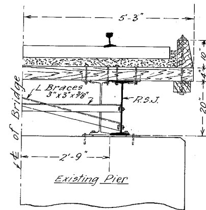
HALF CROSS SECTION SCALE 1/2" = 1'-0"
