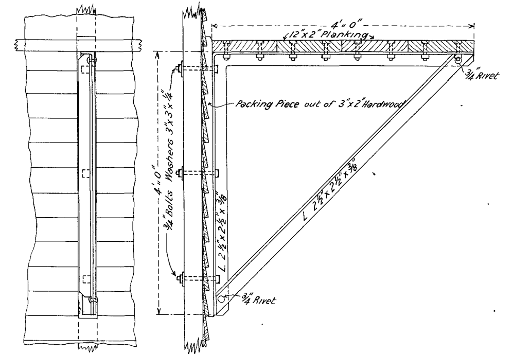
— Detail of Bracket — — Scale 1" = 1' —
