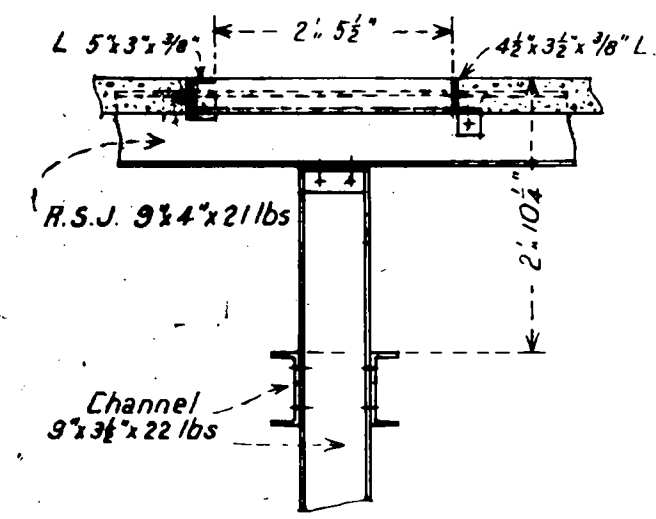
— Section A-A through Floor —
