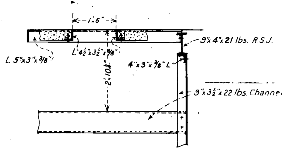
— Section B-B through Floor —
