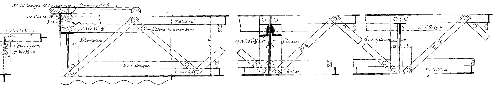
Detail of Girder & Screen Scale 1/2" = 1'-0"
