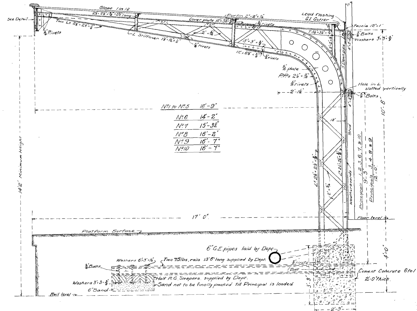
Principal Scale 1/2" = 1'-0"
