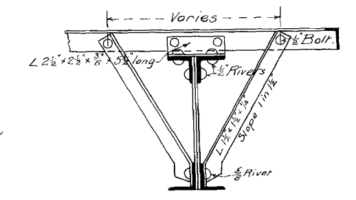
Stiffener to Purlin Scale 1/2" = 1'-0"
