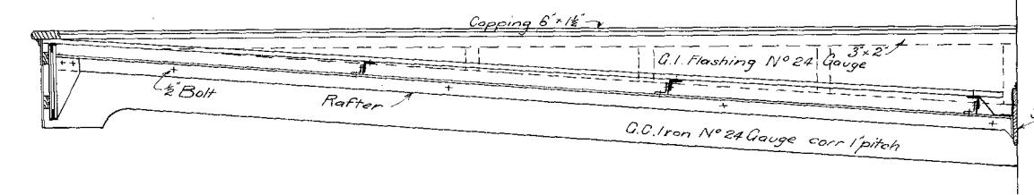
End Rafter Scale 1/2" = 1'-0"
