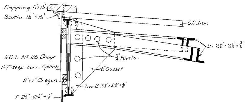
End of Principal Scale 1/2" = 1'-0"
