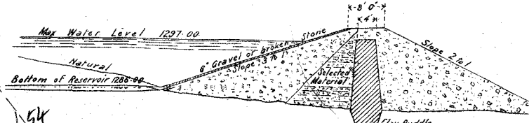
Section through Dam
