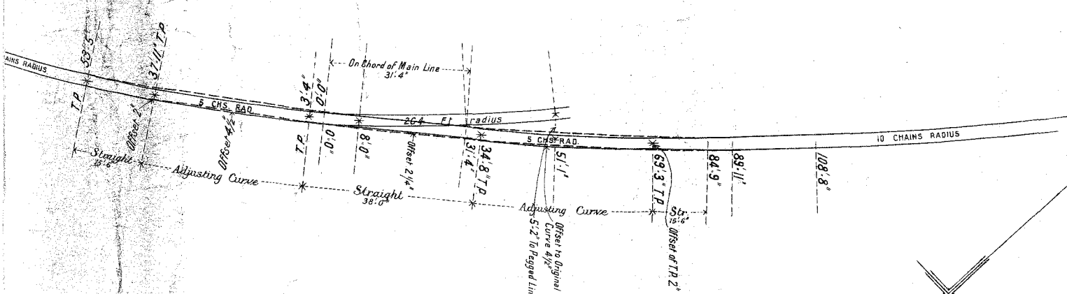
Plan showing Adjustment of Main Line
