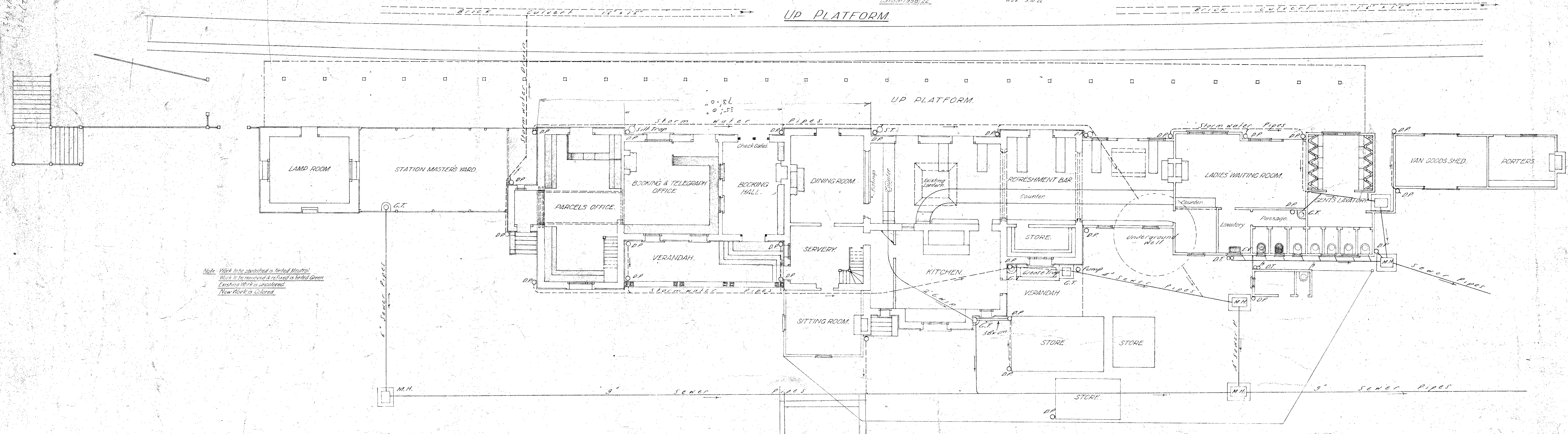
PLAN OF EXISTING BUILDINGS ON UP PLATFORM.
