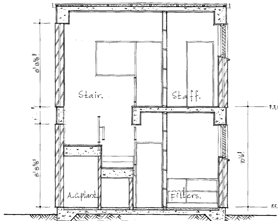
CROSS SECTION : 1/4" = 1'0"
