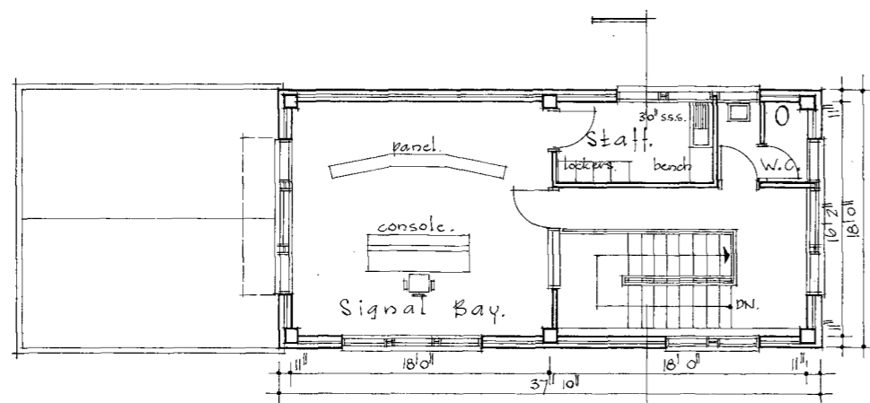
1/8" = 1'0" : First floor.
