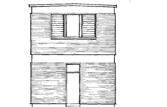
EAST ELEVATION:
