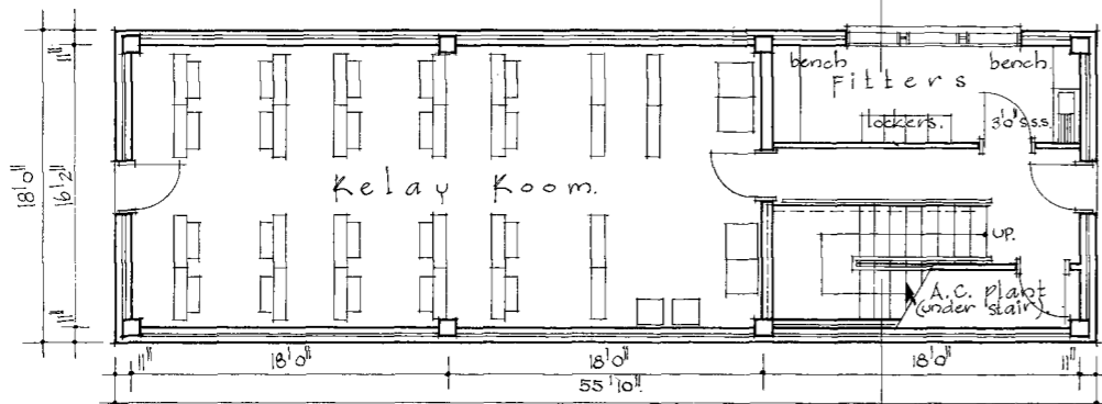
1/8" = 1'0" : Ground floor.
