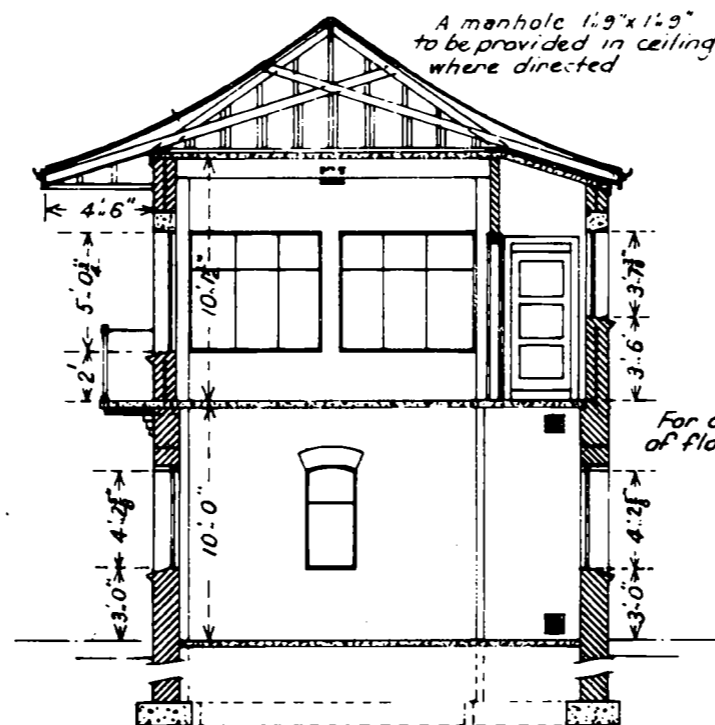
CROSS SECTION
