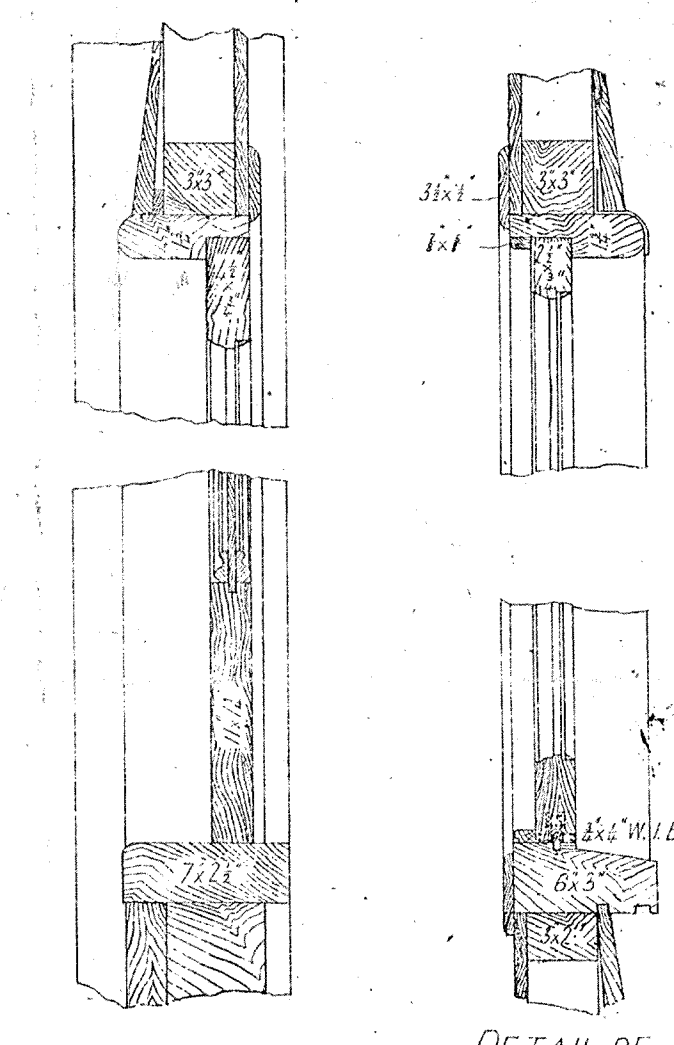
SECTION OF VENTILATOR
