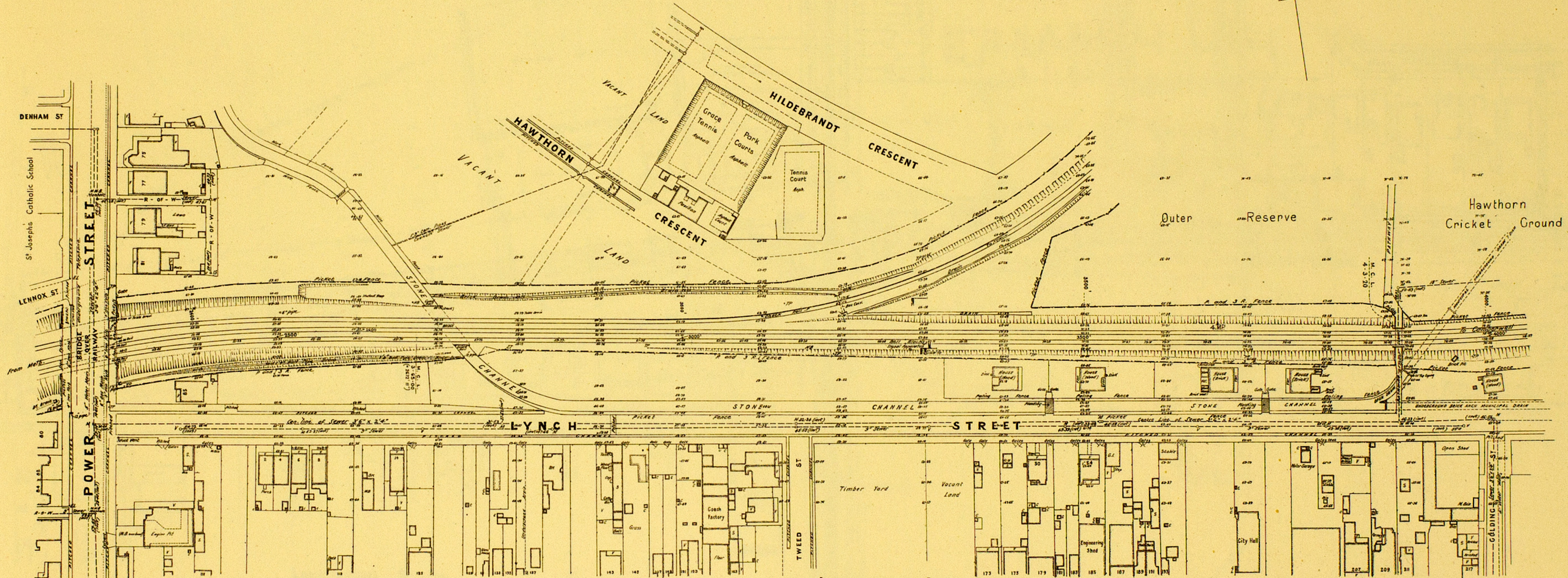
LONGITUDINAL SECTION SCALES (Hor 100-1 inch Ver 25-1 inch
